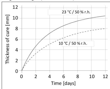
Schema 1: Curing speed of Sikaflex®-515
